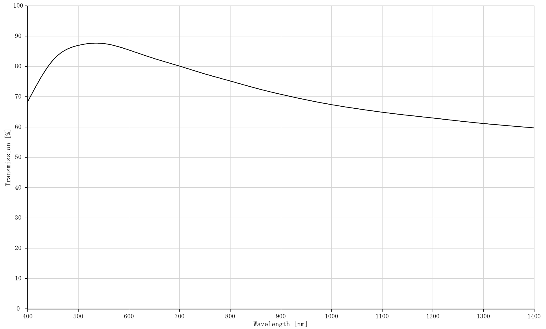
LM35EC-IR Transmission
